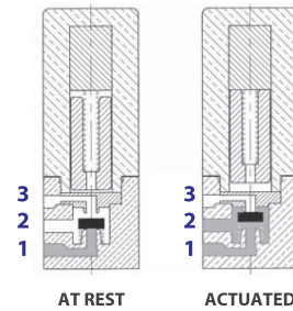
NORMALLY CLOSED (NC) 3/2
