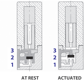
NORMALLY OPEN (NO) 3/2
